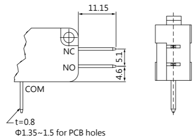
PCB terminal K TYPE
