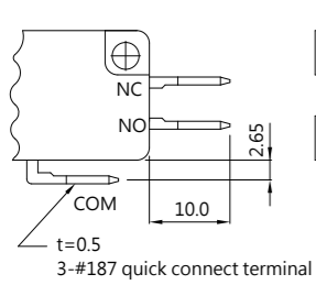
Quick connect terminal 187 Series D TYPE
