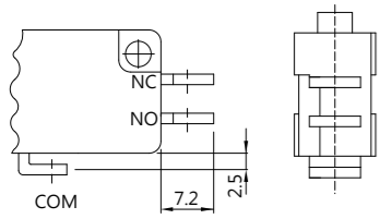
Solder terminal A TYPE
