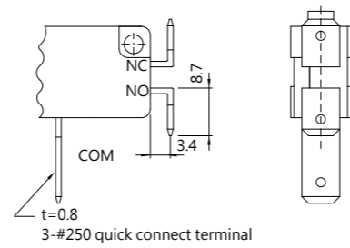
Quick connect terminal 250 Series F TYPE
