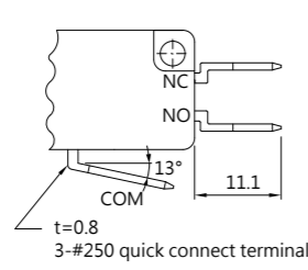
Quick connect terminal 250 Series E TYPE
