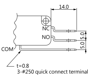
Quick connect terminal 250 Series G TYPE
