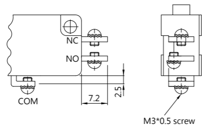
Screw terminal B TYPE
